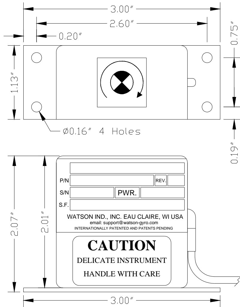
Figure 1: ARS-C142-1A Dimensions
