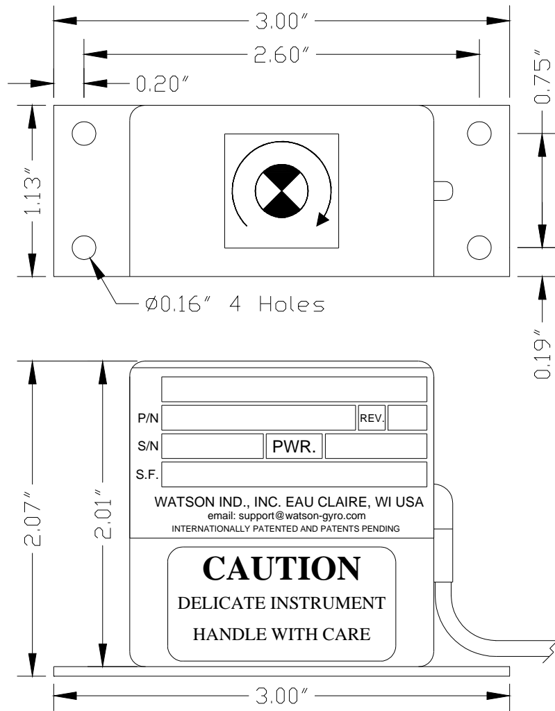
Figure 1: ARS-C132-1A Dimensions
